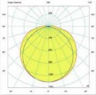
Photometric diagrams
